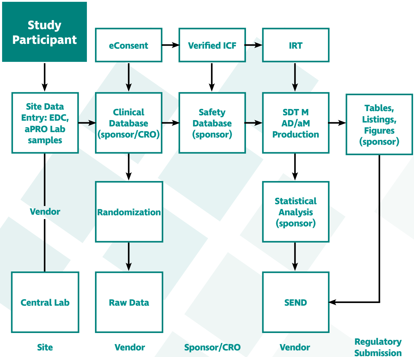
Figure 1. An example Data Flow Diagram
